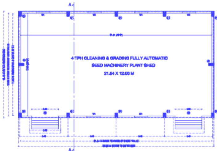
FULLY AUTOMATIC SEED MACHINERY PLANT SHED PLAN
